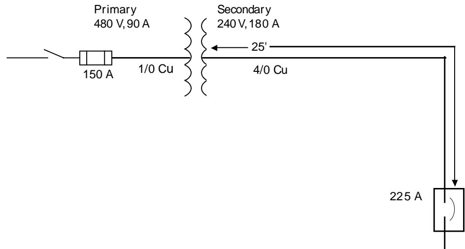
Figure 11: Secondary Conductors Not Over 25 Feet
