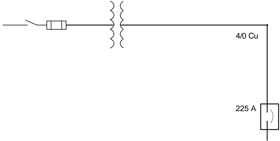
Figure 15: Overload Protection—Single Overcurrent Device
